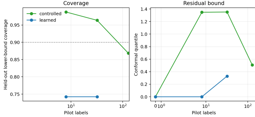
Figure 10: Residual lower-bound calibration diagnostics.
