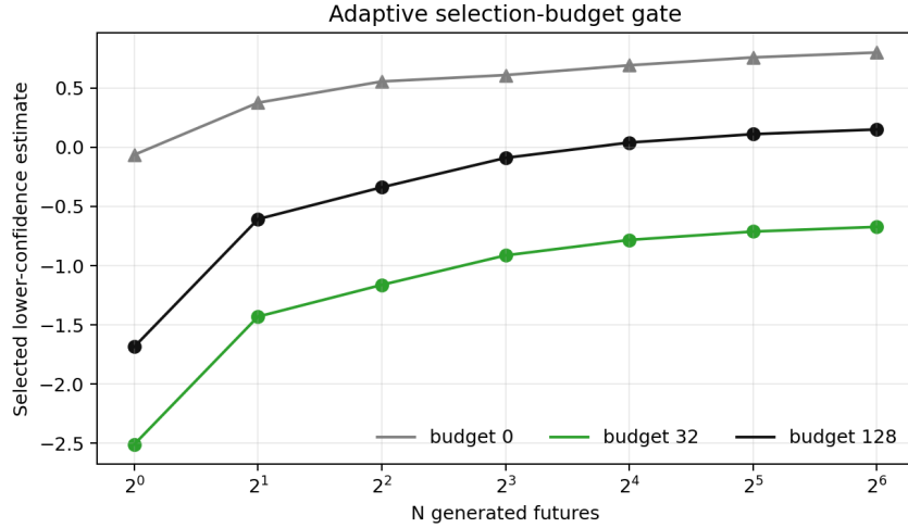
Figure 9: Adaptive selection-budget gate decisions with explicit reason codes.
