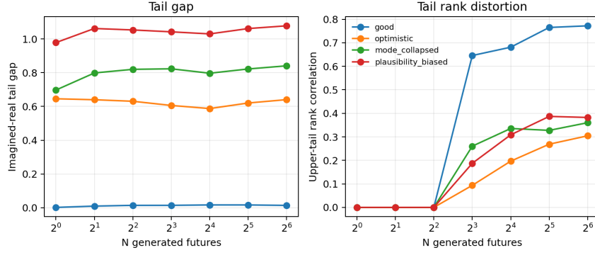
Figure 8: Selected-tail diagnostics, including imagined-real tail gap and upper-tail rank correlation.
