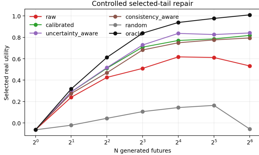
Figure 7: Raw scoring compared with calibrated, uncertainty-aware, consistency-aware, random, and oracle scoring.
