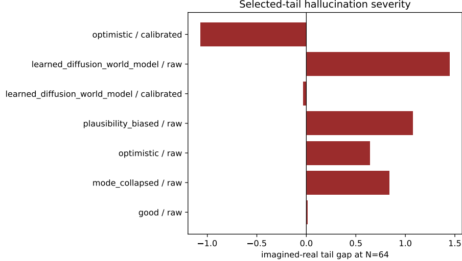
Figure 3: V3 selected-tail failure landscape at N = 64 . The raw learned diffusion-world scorer has tail gap 1.447 and selected real utility -0.782, while the controlled optimistic raw scorer has tail gap 0.641.
