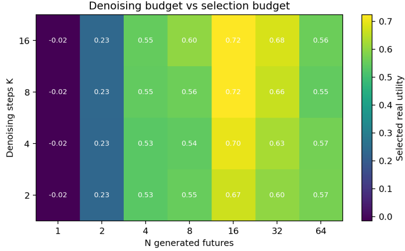
Figure 6: Denoising budget K and selection budget N are varied separately.
