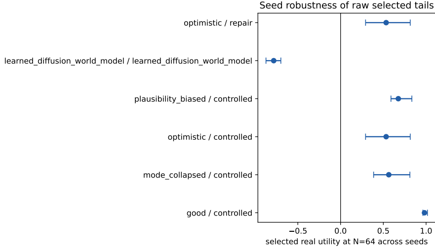
Figure 12: V3 seed robustness at raw N = 64 . Points show mean selected real utility and bars show min/max over seeds.
