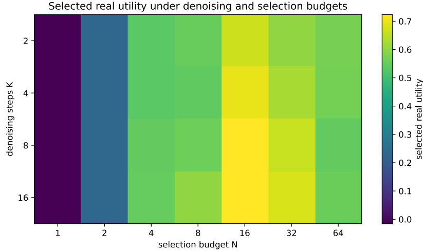
Figure 13: V3 denoising-versus-selection heatmap. Rows vary denoising steps K and columns vary selection budget N ; colors show selected real utility.
