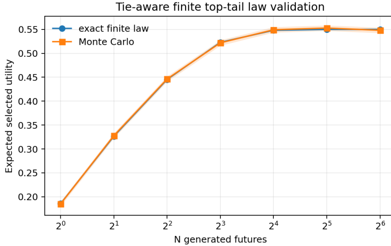
Figure 5: Finite tie-aware law versus Monte Carlo selection. The maximum absolute validation error is 0.0028.
