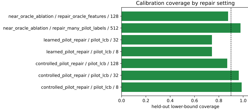
Figure 14: V3 lower-bound coverage by repair setting. The dashed line marks the nominal 0.9 confidence level.
